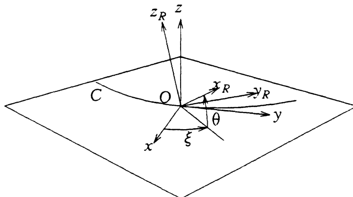
Fig.A5.1. Curve C , local axes Oxyz and rotated axes Ox_R y_R z_R .
