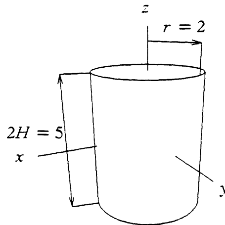
Fig.8.1. Cylinder with radius r=2 , height 2H=5 .
