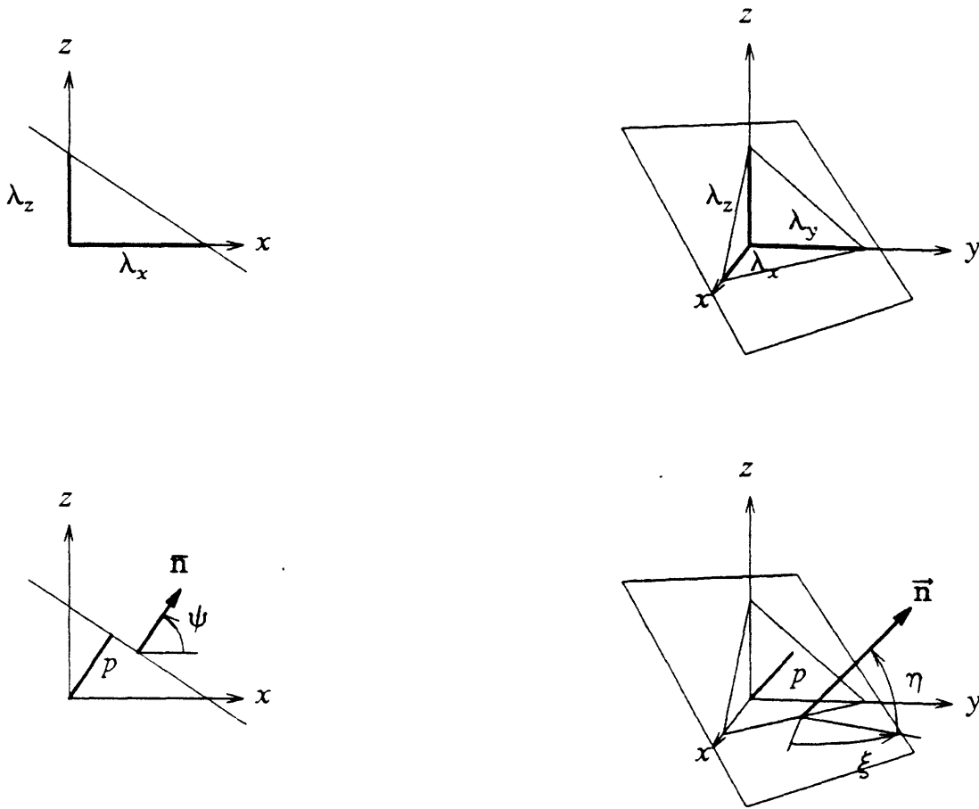
Fig.3.2. Tangential Coordinates.
