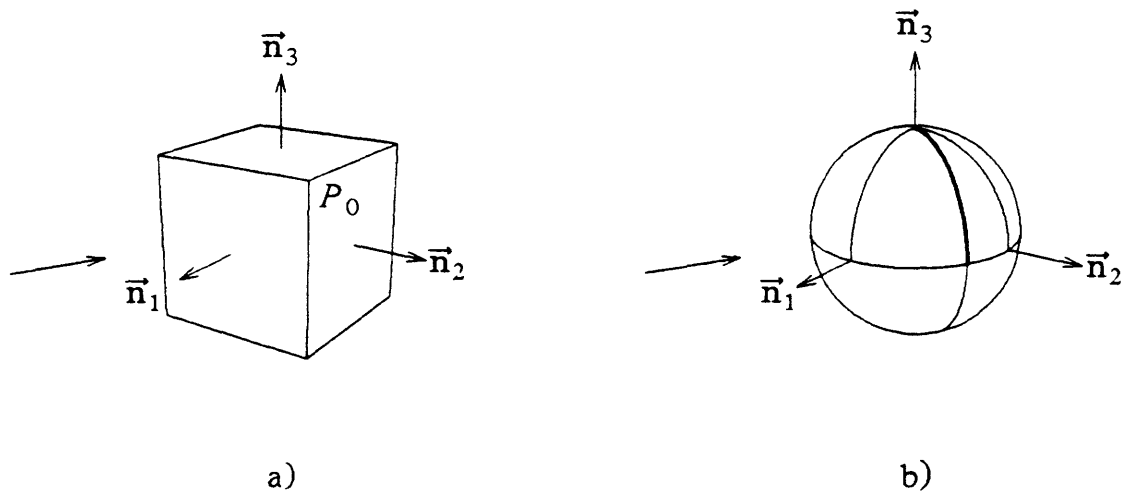
Fig.7.12. Silhouette of a cube corner. a) Corner. b) Gaussian image, with a slice corresponding to the silhouette with the largest exterior corner angle.
