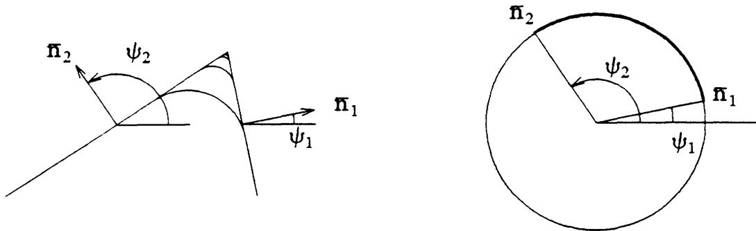
Fig.7.2. Curve with a Corner. a) Sequence of curves approximating the corner. b) Gaussian circles.
