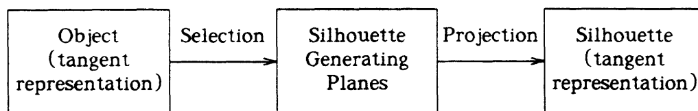
Fig.4.5. Silhouette Construction with Tangential Representations.
