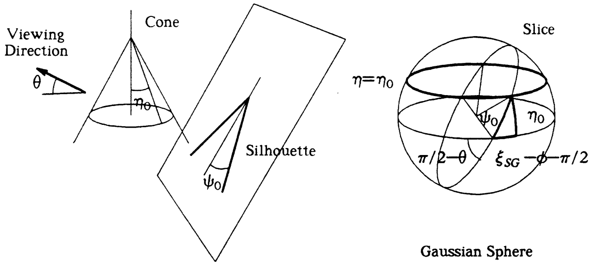
Fig.4.8. Silhouette of the Cone and Gaussian Sphere.
