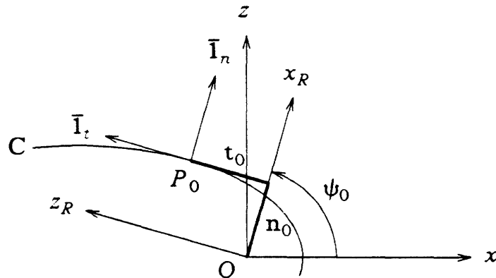
Fig.5.2. VST of P_0 as Coordinates in the Rotated Frame.
