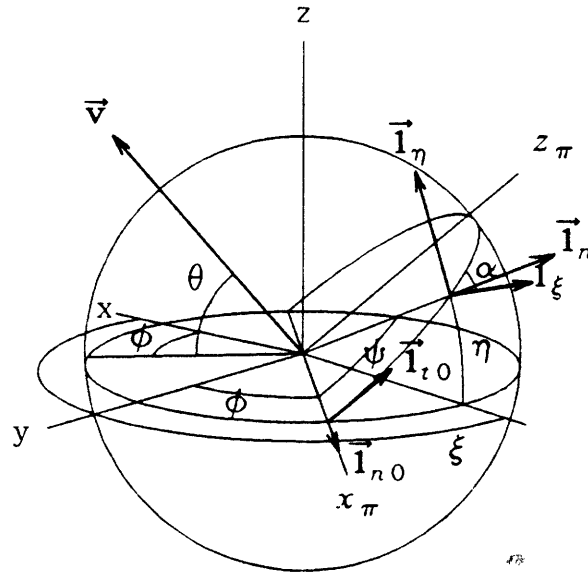
Fig.6.4. Illustration of the Composition of Rotations.
