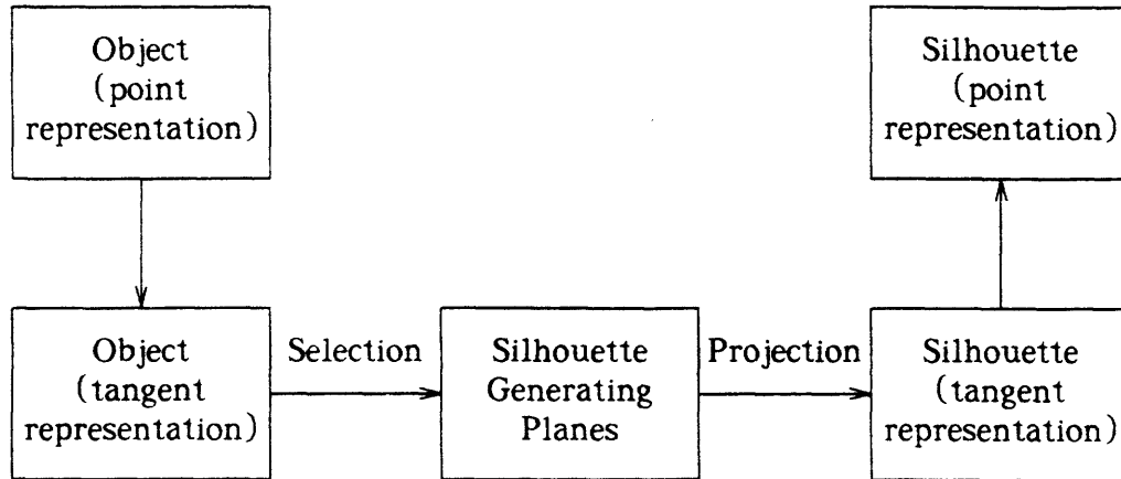
Fig.4.6. Silhouette Construction with Conversion to Tangential Representation.
