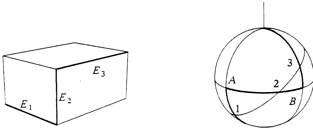
Fig.8.18. Three Silhouette Edges and the corresponding CT
