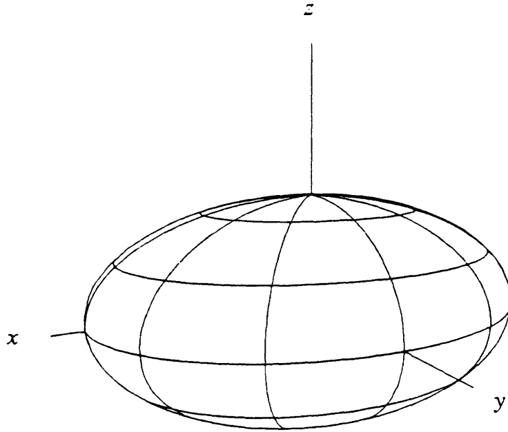
Fig.A1.5. Ellipsoid with semi-axes a=4, b=3, c=2 .
