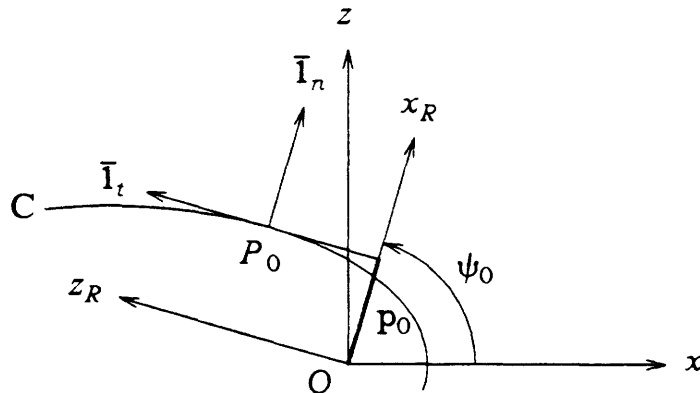
Fig.5.1. Tangent to the curve C at P_0 and normal distance p_0 .
