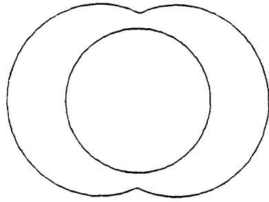
Profile of 3-D ST (exterior)
