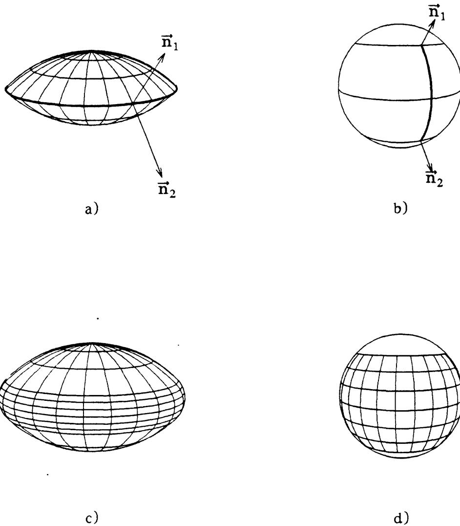
Fig.7.5. Surface with a Curved Edge
