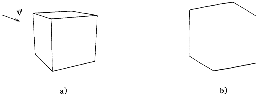
Fig.1.4. Cube and its Silhouette for the Viewing Direction \vec{v} .
