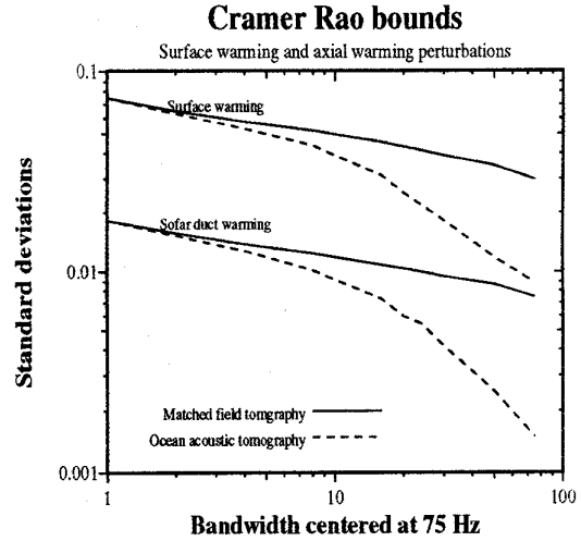
Figure 2: Lower bounds for matched field tomography (solid line) and (ocean acoustic tomography (dashed line).
